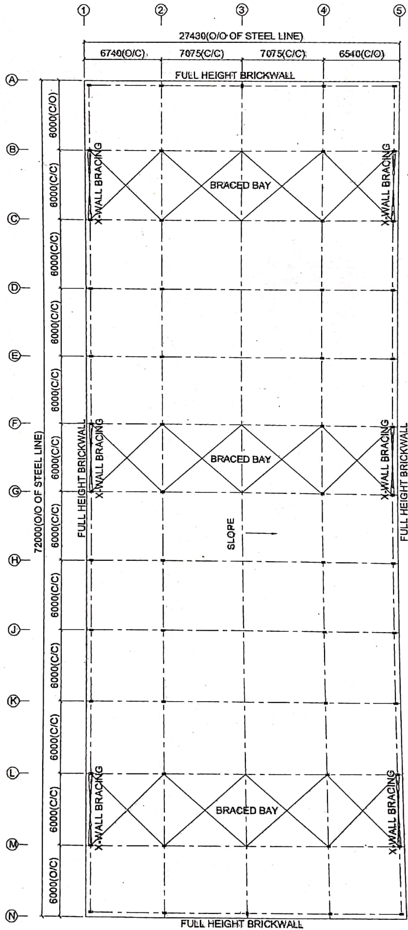
PROPOSED PLAN
